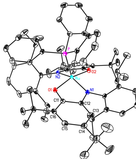
Fig. 4 Thermal ellipsoid plot of (Diso) _2\text{Ru}(\text{PPh}_3)_2 \cdot 2 \text{CH}_2\text{Cl}_2 , with hydrogen atoms and lattice solvent omitted for clarity.
