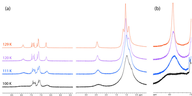
Fig. 3 ^1\text{H} NMR spectra of trans -(Diso) _2\text{RuCl}_2 in 80% \text{CF}_2\text{Cl}_2 /20% \text{CDFCl}_2 (400 MHz). (a) Full spectrum. (b) Downfield region, showing the decoalescence of the iminoxolene resonance at \delta 7.9 ppm.
